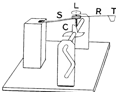
FIG. 10.—THE SPRING-TAPPER
