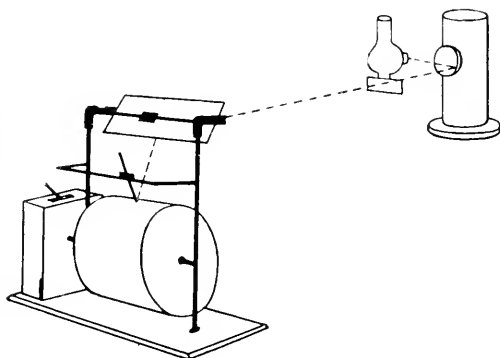
FIG. 8.—RESPONSE RECORDER
