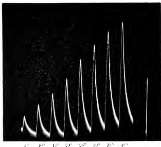
FIG. 83.—RECORDS OF RESPONSES IN TIN WITH INCREASING STIMULI, AMPLITUDES OF VIBRATION FROM 5^{\circ} TO 40^{\circ}
